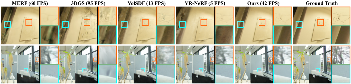
Figure 4.8: ScanNet++ [213] . 3D Gaussian splatting [81] struggles with specular surfaces such as whiteboards ( above ) and far-field content ( below ). Our method performs best qualitatively while maintaining a real-time frame rate.
