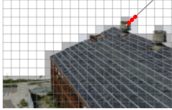
Guided Sampling
