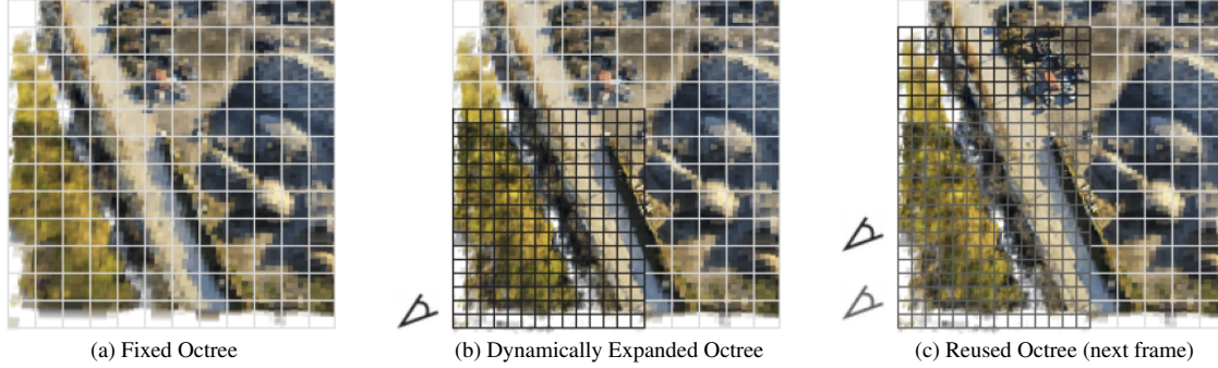
Figure 2.4: Mega-NeRF-Dynamic . Current renderers (such as Plenocree [216]) cache precomputed model outputs into a fixed octree, limiting the resolution of rendered images (a). Mega-NeRF-Dynamic dynamically expands the octree based on the current position of the fly-through (b). Because of the temporal coherence of camera views, the next-frame rendering (c) can reuse of much of expanded octree.
